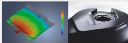
3D Mold Flow Simulation 3D流道模擬分析
